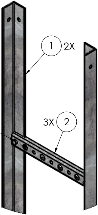
DETAIL A SCALE 1 : 7
